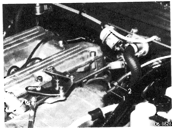
Vacuum connection on engine 110.98
