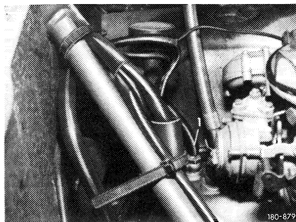
Vacuum connection on engine 130.923
