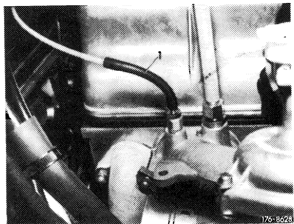
Vacuum connection on engine 115
