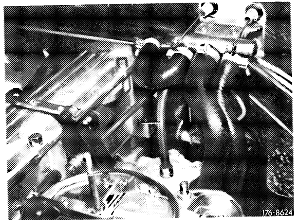
Vacuum connection on engine 110.92
