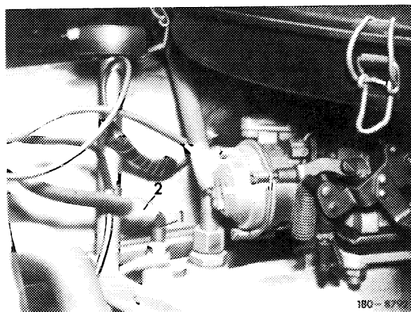
Vacuum connection on engine 130.920
