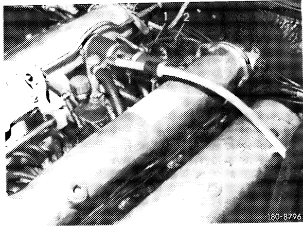
Vacuum connection on engine 100.981
