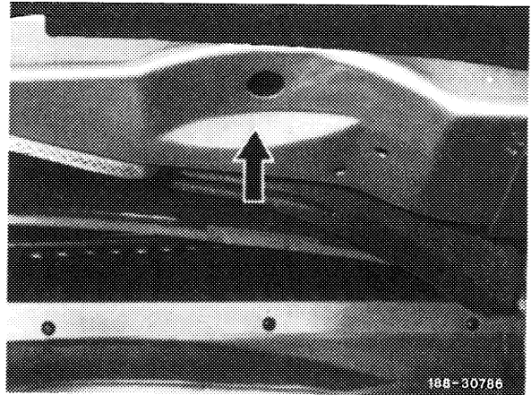
Fig. 88/3 Depression for brake booster clearance
